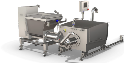
scanEmul 175 screw hopper fed
