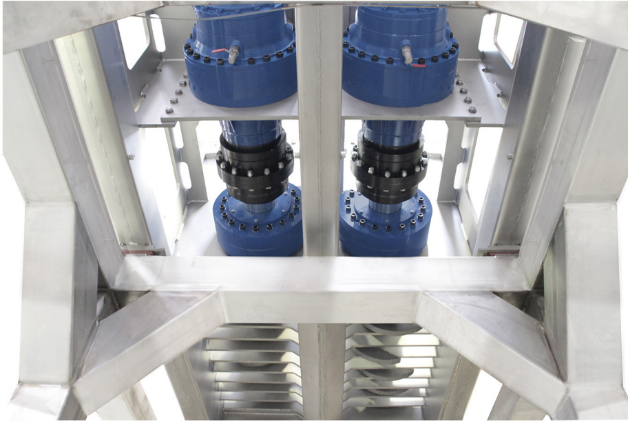
Top picture: Heavy Duty safety clutch claw and gear box. Bottom picture: The rotary and stationary claw design comes in two versions.
