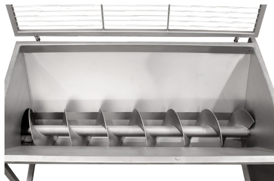
Infeed hopper shown with safety guard/grill in cleaning and inspection position.
