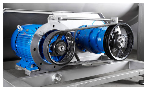
Pump transmission.
